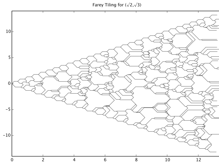
FIGURE 1. This picture, produced by Y. Cheung, represents dynamics of the Weyl chamber flow.
