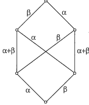
FIGURE 1: The Bruhat ordering of W(A_2) .
