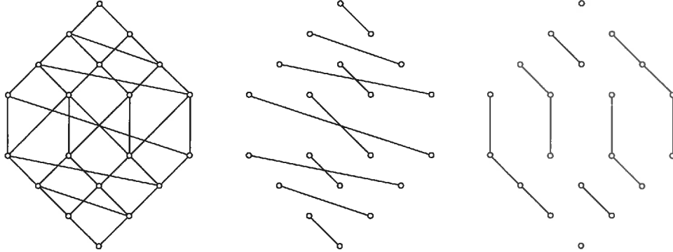
FIGURE 2: The Bruhat ordering of a W -orbit in \mathcal{A}_4 .
