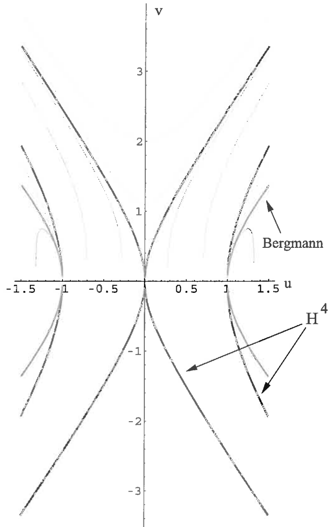
Figure 2: The phase plane for the first-order system of equation (83). The heavy blue hyperbola corresponds to the Bergmann flow, and the three heavy red hyperbolae to H^4 flows. The discussion of other flows is analogous to that for \Lambda > 0 ; some representative examples are depicted.
