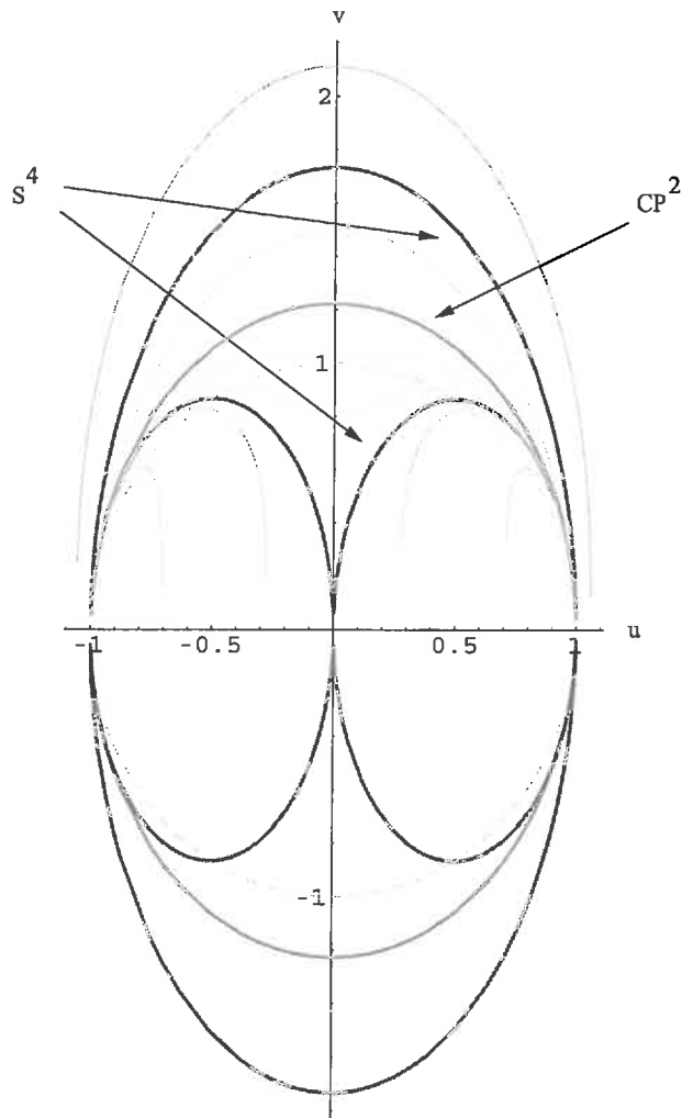
Figure 1: The phase plane for the first-order system of equation (72). The heavy blue ellipse corresponds to the \mathbb{CP}^2 flow, and the three heavy red ellipses to S^4 flows. The dashed green circle is u^2 + v^2 = 1 ; all solutions that cross this do so horizontally. To label distinct metrics it is sufficient to consider flows lying within the positive quadrant. We label qualitatively similar flows by A, B, C and D, which indicate the regions they occupy and their initial points. Thus the regions A, B and C indicate starting-points for solutions on the v axis. Region A ranges from v = 0 to the intersection of the \mathbb{CP}^2 ellipse with the v axis. Region B ranges from this intersection to the intersection of the outer ellipse (the S^4 solution (70)) with the v axis. Region C ranges from this point to v = +\infty . Region D denotes (singular) starting points on the u axis for solutions, in the range 0 < u < 1 . For clarity we have plotted complete ellipses for the S^4 and \mathbb{CP}^2 special cases, but only flows in the upper half-plane for the other representative examples.
