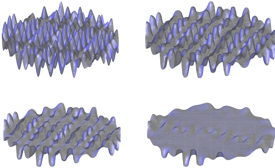
FIG. 5.4. Solution u for the initial data (5.3) at times 0.0 , 1.4 \times 10^{-6} , 3.5 \times 10^{-6} and 6.3 \times 10^{-6} .
