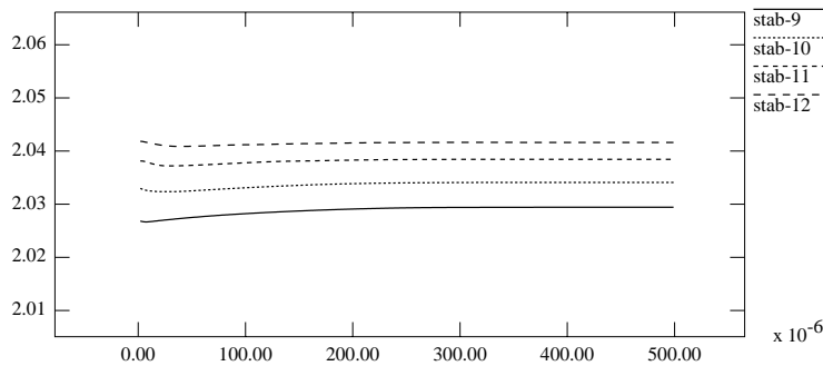
FIG. 5.3. Quantity (5.2) for the singular example from Figure 5.1 as a function of time t \in [0, 0.0005] for several spatial discretization levels.
