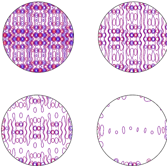
FIG. 5.4. Solution u for the initial data (5.3) at times 0.0 , 1.4 \times 10^{-6} , 3.5 \times 10^{-6} and 6.3 \times 10^{-6} .
