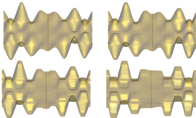
FIG. 5.7. The solution from Figure 5.6 shown as graph.
