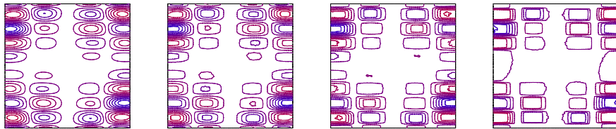
FIG. 5.8. Level lines of the solution from Figure 5.7.
