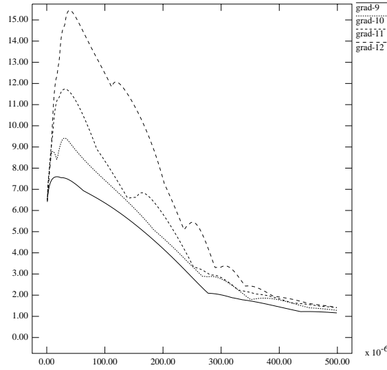
FIG. 5.2. Lipschitz-norm of the discrete solution (vertical axis) plotted as a function of time t \in [0, 0.0005] for the initial function from (5.1) for different spatial discretization levels.
