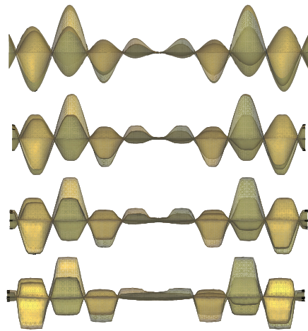
FIG. 5.6. Anisotropic surface diffusion for the initial function (5.5) with anisotropy (5.4), view from the x_1 axis. Time steps 0, 10, 50, 200.
