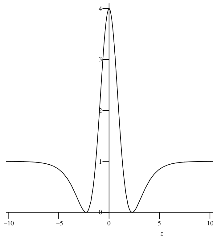
Figure 3.5. A solitary wave with compressive and rarefactive regions for m = \frac{1}{2} , n = 0 .
