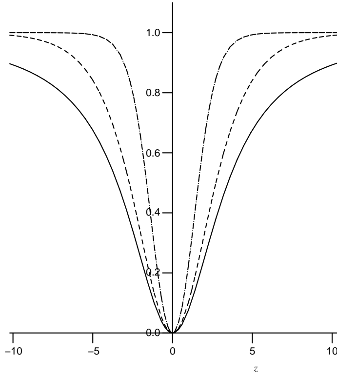
Figure 3.3. Solitary waves for m = 2 , n = 2 , which are exponential for c = -2 ( - \cdot - ) and c = 3 ( - - - ) and algebraic when c = 2 ( — ).
