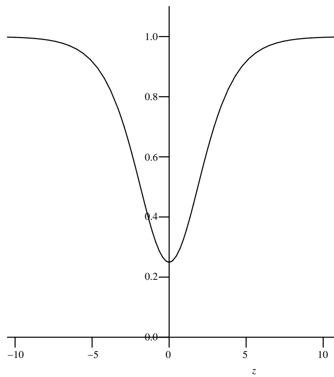
Figure 3.2. A compressive solitary wave for m = 0 , n = -1 when c = -2 .
