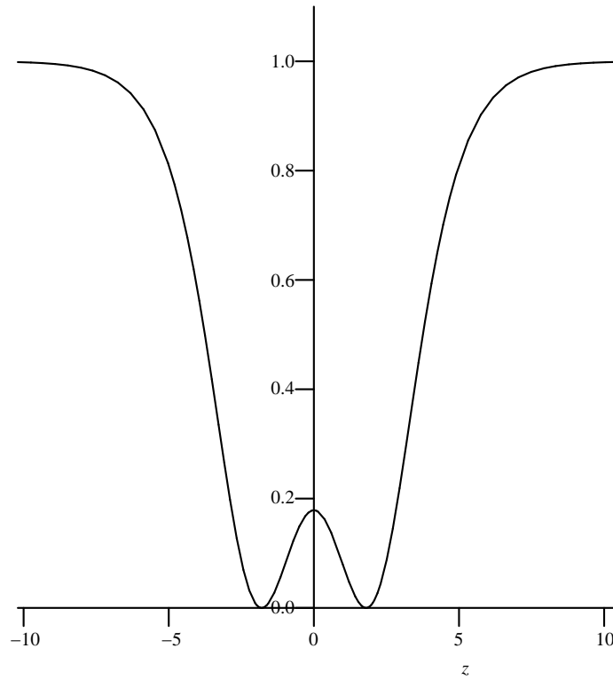
Figure 3.4. An oscillatory solitary wave for m = -\frac{1}{2} , n = -\frac{1}{2} when c = -6 .
