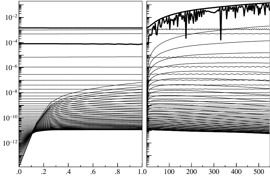
Figure 1: Actions, total energy (upper bold line), and momentum (lower bold line) along the numerical solution of DOPRI5, average CFL number 1.075.
