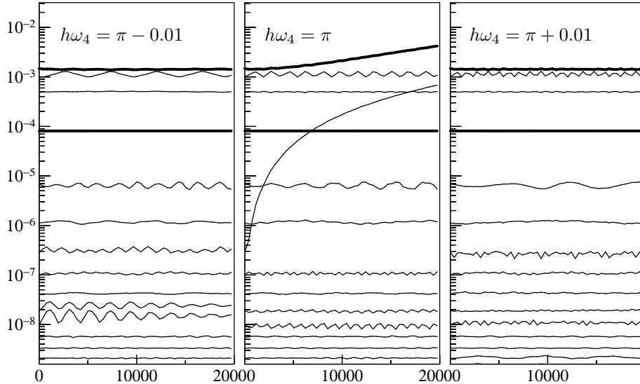
Figure 3: Illustration of numerical resonance.
