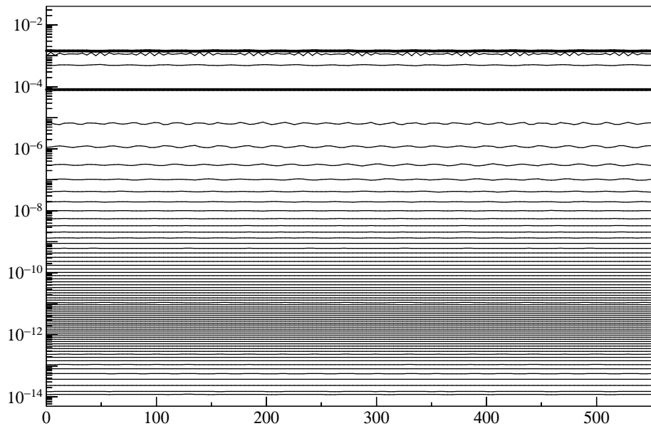
Figure 2: Actions, total energy (upper bold line), and momentum (lower bold line) along the numerical solution of the trigonometric integrator (19) with \psi = \text{sinc} and \phi = 1 for the CFL number h\omega_M \approx 6.4 .
