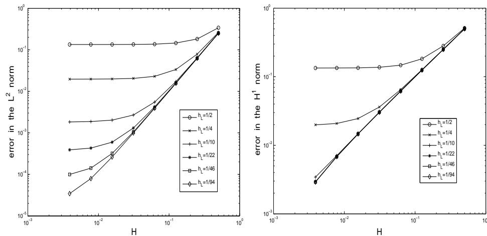
FIG. 5.4. FE-HMM : : macromesh refinement for fixed micro mesh h_L = 1/2, 1/4, 1/10, 1/22, 1/46 .
