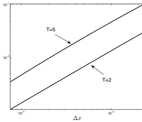
Figure 5: L^1 -error of the centered scheme at T = 2 and T = 5 applied to the single-peakon problem with initial data (22) where x_0 = 0, a = 6, c = 1 .
