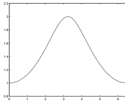
Figure 3: Smooth periodic traveling wave.
