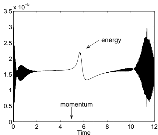
Figure 10: Conservation of momentum (27) and energy (28) for the second multi-symplectic formulation, \Delta x = 0.0133 , \Delta t = 0.0024 .
