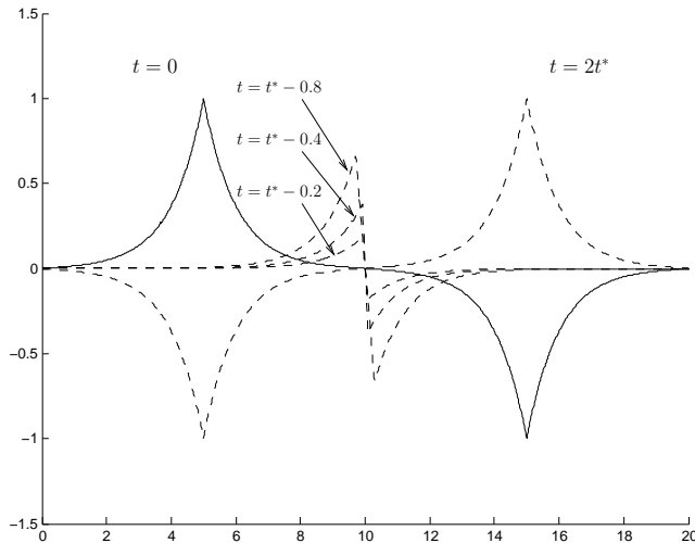
Figure 1: Symmetric peakon-antipeakon collision.
