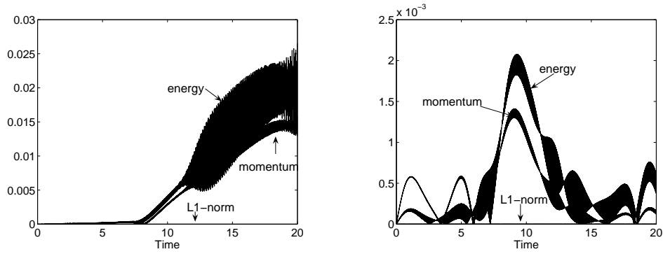
Figure 2: Conservation properties of scheme (19) (left) and the scheme based on centered splitting (20) (right) for smooth initial data.
