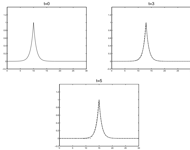
Figure 4: Snapshots of the peakon solution and the numerical solution given by (20).
