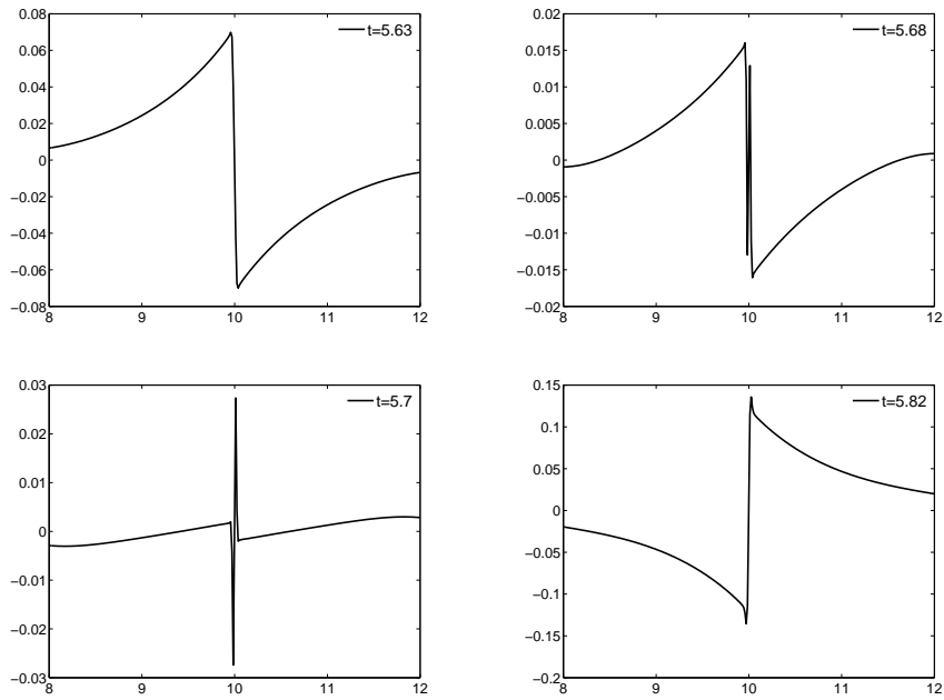
Figure 8: Snapshots showing the collapse and resurrection of an antisymmetric peakon collision, \Delta x = 0.0133 , \Delta t = 0.0024 .
