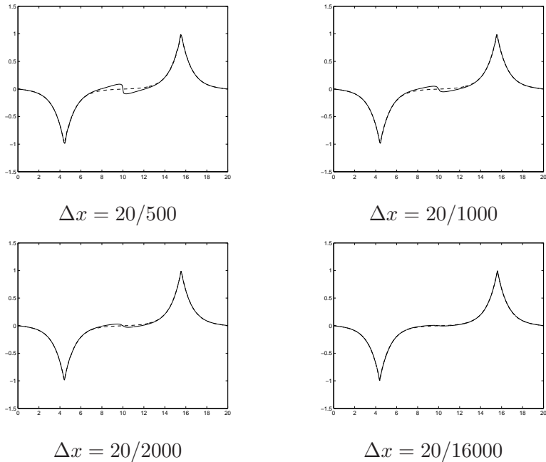
Figure 7: Plot of the computed solution and the exact solution (in dash line) at time t=12 .
