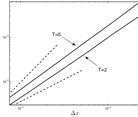
Figure 6: L^1 -error of the centered scheme at T = 2 and T = 5 applied to the single-peakon problem with initial data (22) using x_0 = 0 , a = 6 , and c = 1 . The dashed lines have slopes 1 and 2.
