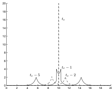
Figure 9: Plot of the energy density, u^2 + u_x^2(x, t) , for the exact solution at different times before collision ( t_c \approx 5.69 is the collision time).
