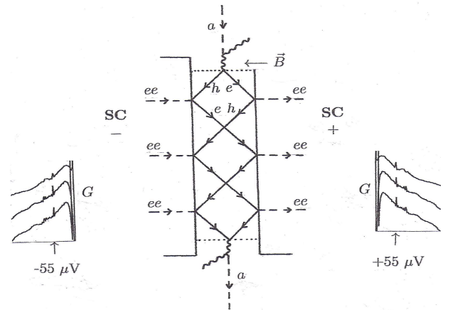
FIG. 2: Axion triggering the transport of n Cooper pairs ee in an S/N/S junction by multiple Andreev reflections, here shown for the example n = 3 . The dotted line corresponds to the normal metal surface. The left and right insets show the shape of the differential conductance curve G(V) as measured by Hoffmann et al. [12] for T = 0.9K, 0.5K, 0.1K (top to bottom), with a peak occurring at \pm 0.055mV .
