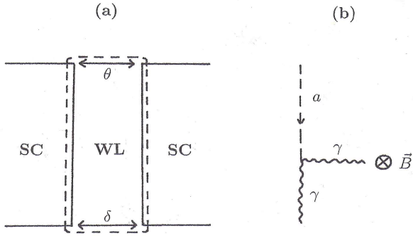
FIG. 1: (a) Closed integration curve (dashed line) over axion and Josephson phase angles in the weak-link region (WL) of a JJ. (b) Feynman graph underlying axion-photon decay in a JJ.
