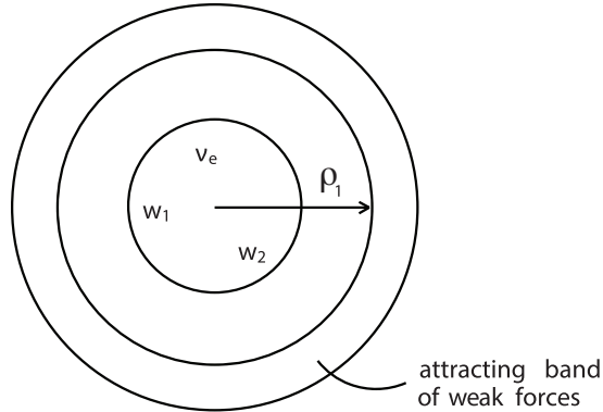
FIGURE 4.1. Electron structure: mediator cloud of an electron
