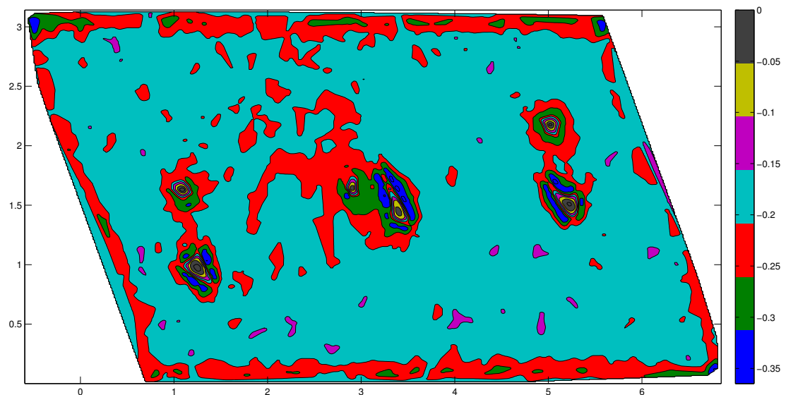
Figure 2: \kappa for the observable g_3 , \beta = 3 for an ensemble of 2000 points. The theoretical expected value is \kappa = -1/6 (azure). See text for description.
