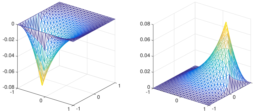
FIGURE 5.1. The mean fields of primal (left) and dual (right) Galerkin solutions in Experiment 1.
