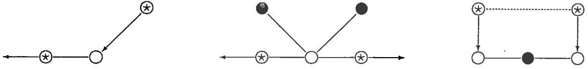
Figure 10: Illustrative pictures for Observations 5.1, 5.2 and 5.3.
