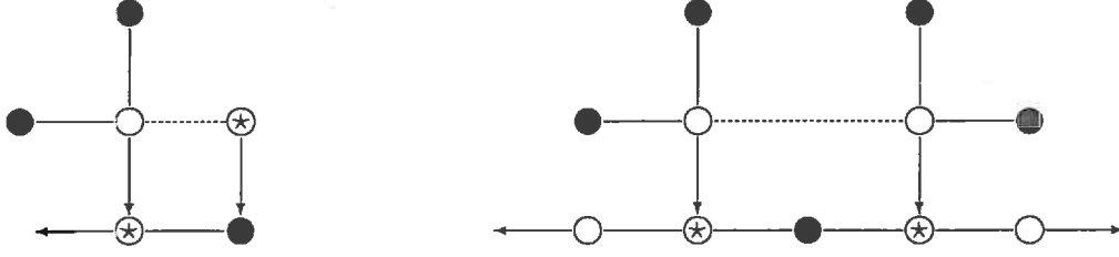
Figure 12: Illustrative pictures for Observations 5.6 and 5.7.
