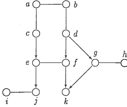
Figure 1: Example of a chain graph from [9].
