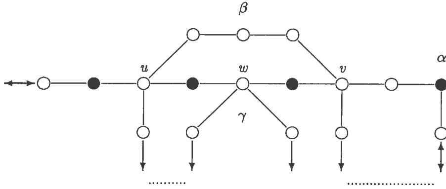
Figure 22: An illustrative picture for the proof of Observation 6.11.
