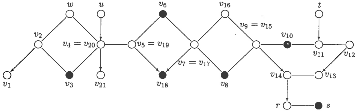
Figure 7: An example illustrating additional graphical concepts.
