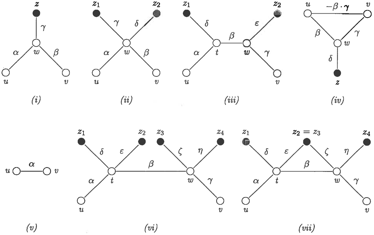
Figure 13: Pictures illustrating Lemma 5.5.
