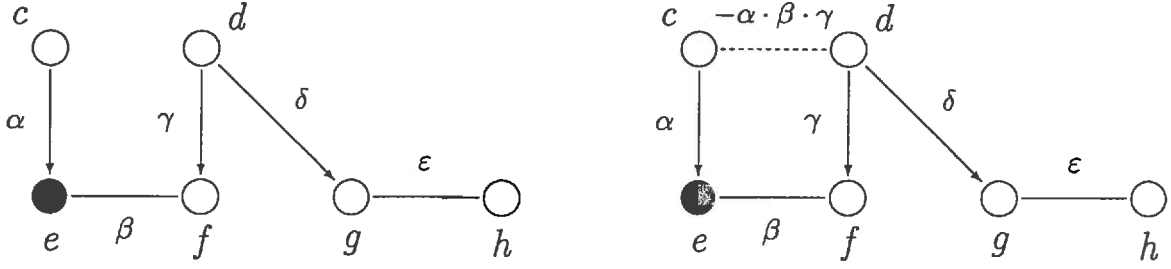
Figure 14: Construction of a Markovian distribution.
