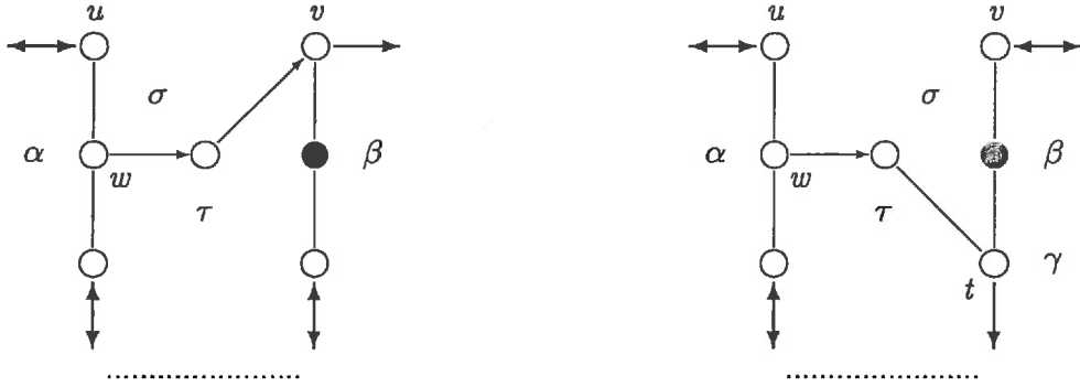
Figure 17: Illustrative pictures for the proof Observation 6.5.
