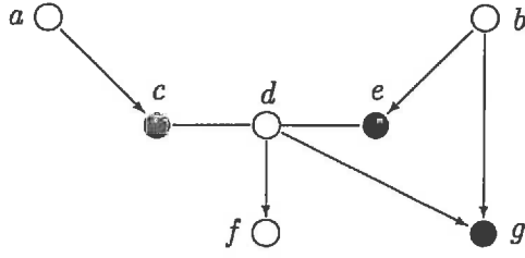
Figure 6: One cannot ignore self-intersecting routes in c-separation.
