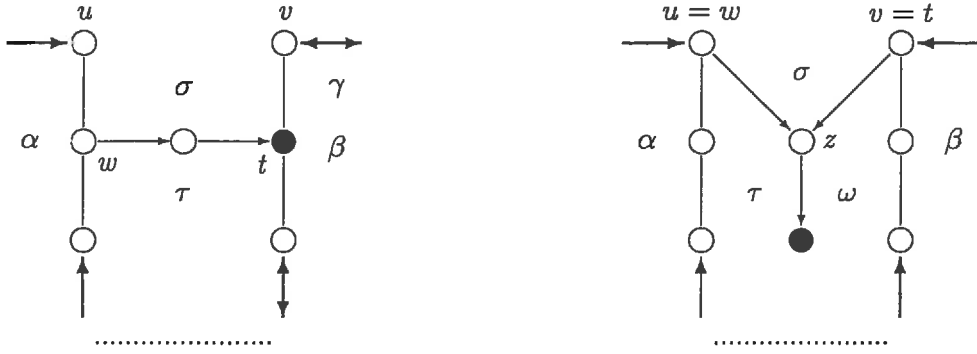
Figure 21: Illustrative pictures for the proofs of Observation 6.9 and Observation 6.10.
