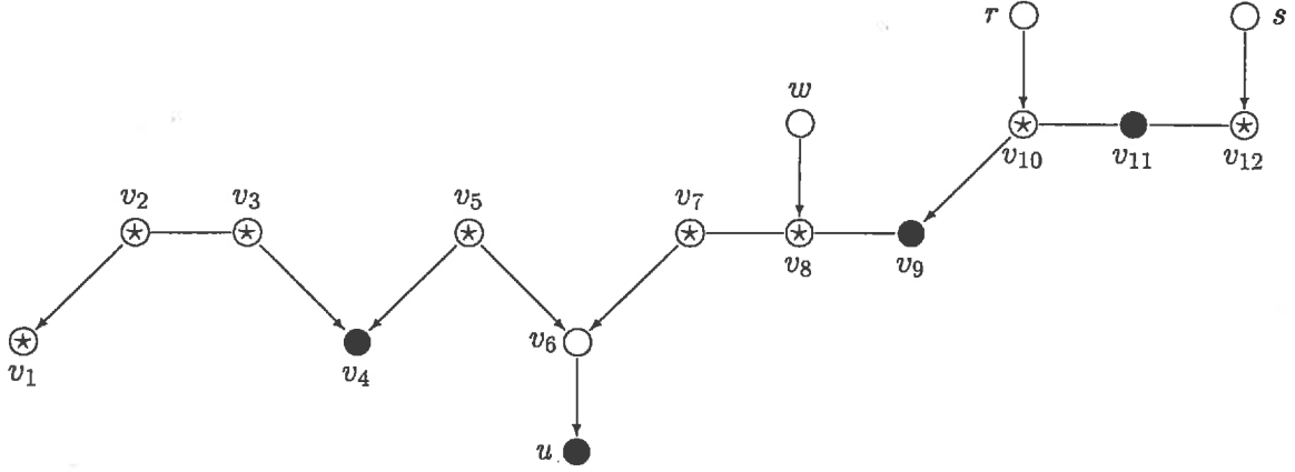
Figure 9: Segments of a trail.
