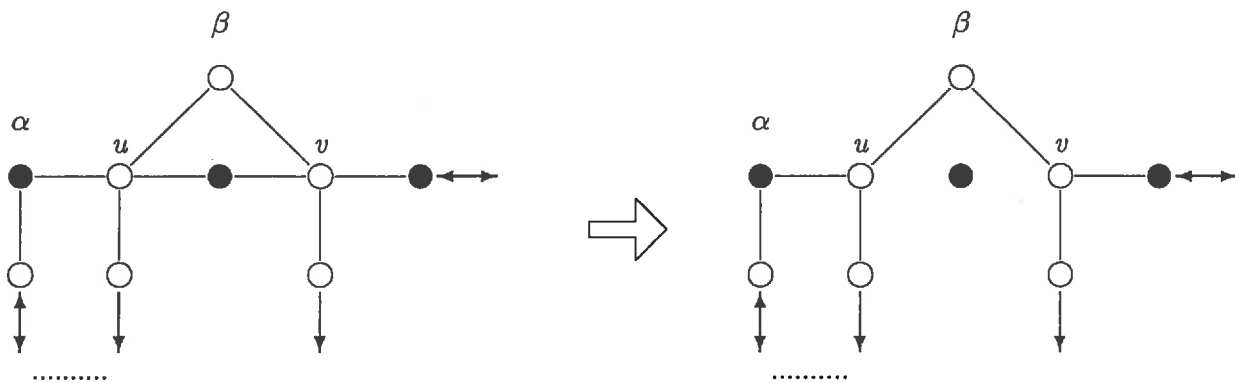
Figure 25: Regularization with respect to free tail-to-tail sections.
