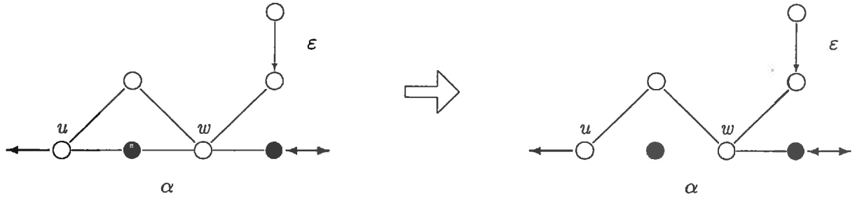
Figure 24: Regularization with respect to free slides.
