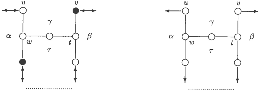
Figure 16: Illustrative pictures for the proofs of Observation 6.3 and Observation 6.4.
