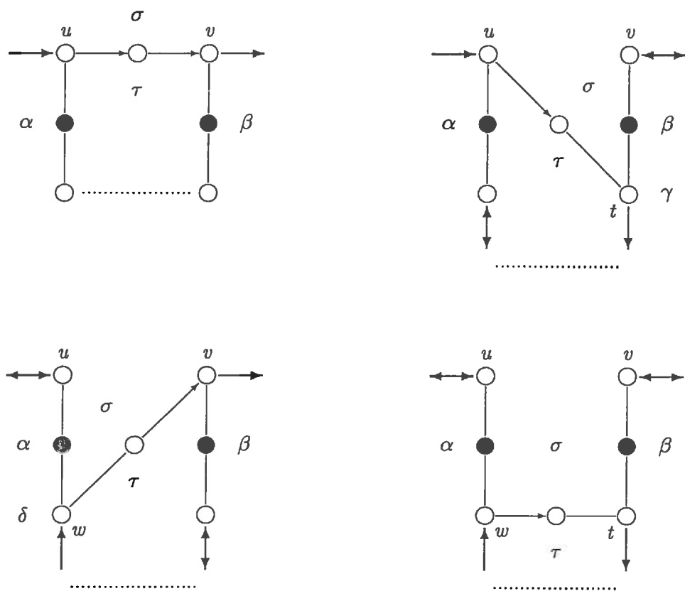
Figure 18: Illustrative pictures for the proof of Observation 6.6.
