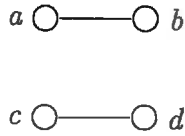
Figure 4: Semigraphoid closures depend on the choice of the input list.
