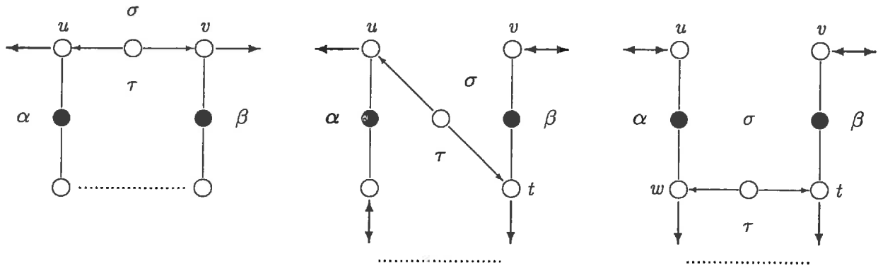
Figure 20: Illustrative pictures for the proof of Observation 6.8.
