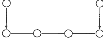
Figure 2: A complex of degree 4.
