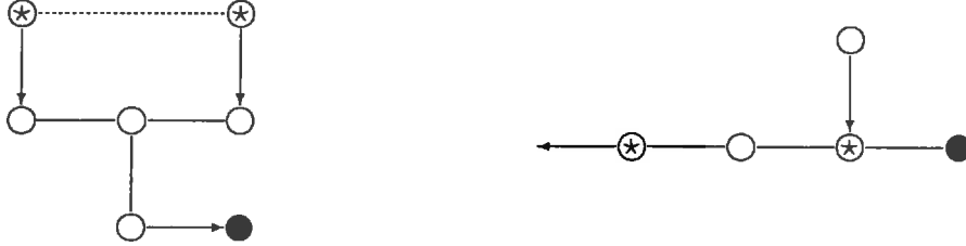
Figure 11: Illustrative pictures for Observations 5.4 and 5.5.
