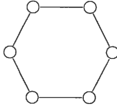
Figure 5: An UG-model having a more complex semigraphoid-generating base.
