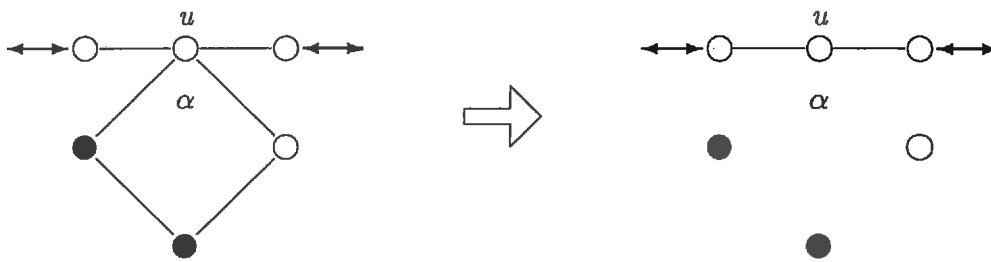
Figure 23: Shortening of sections.
