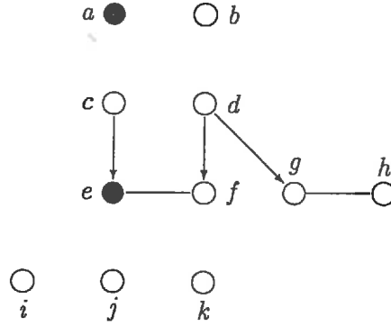
Figure 8: An example of the chosen subgraph.
